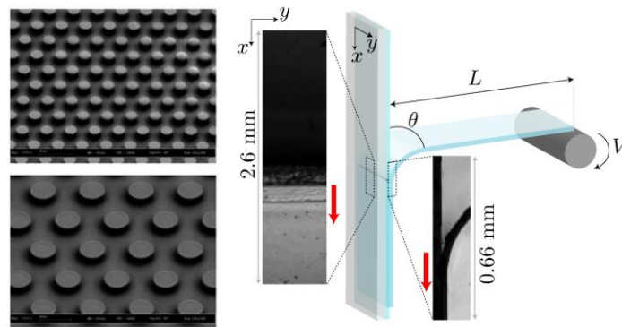
Left: Micro-patterned substrates. Right: Peeling experiment
